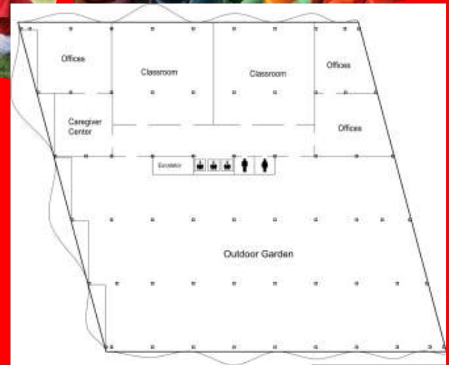
4th Floor
