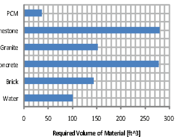
Required Volume of Material To Heat Library Space (54,054 ft 3 )
