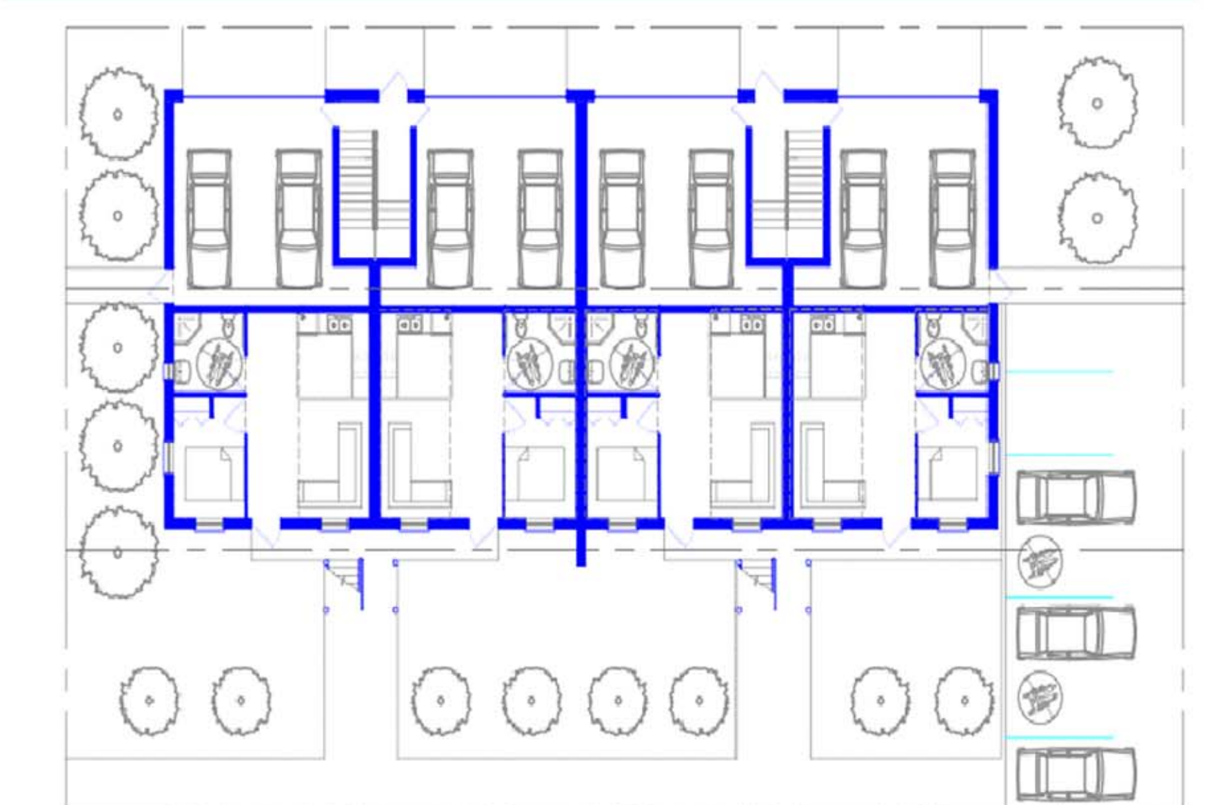
Site Plan- Grade level floor plan
