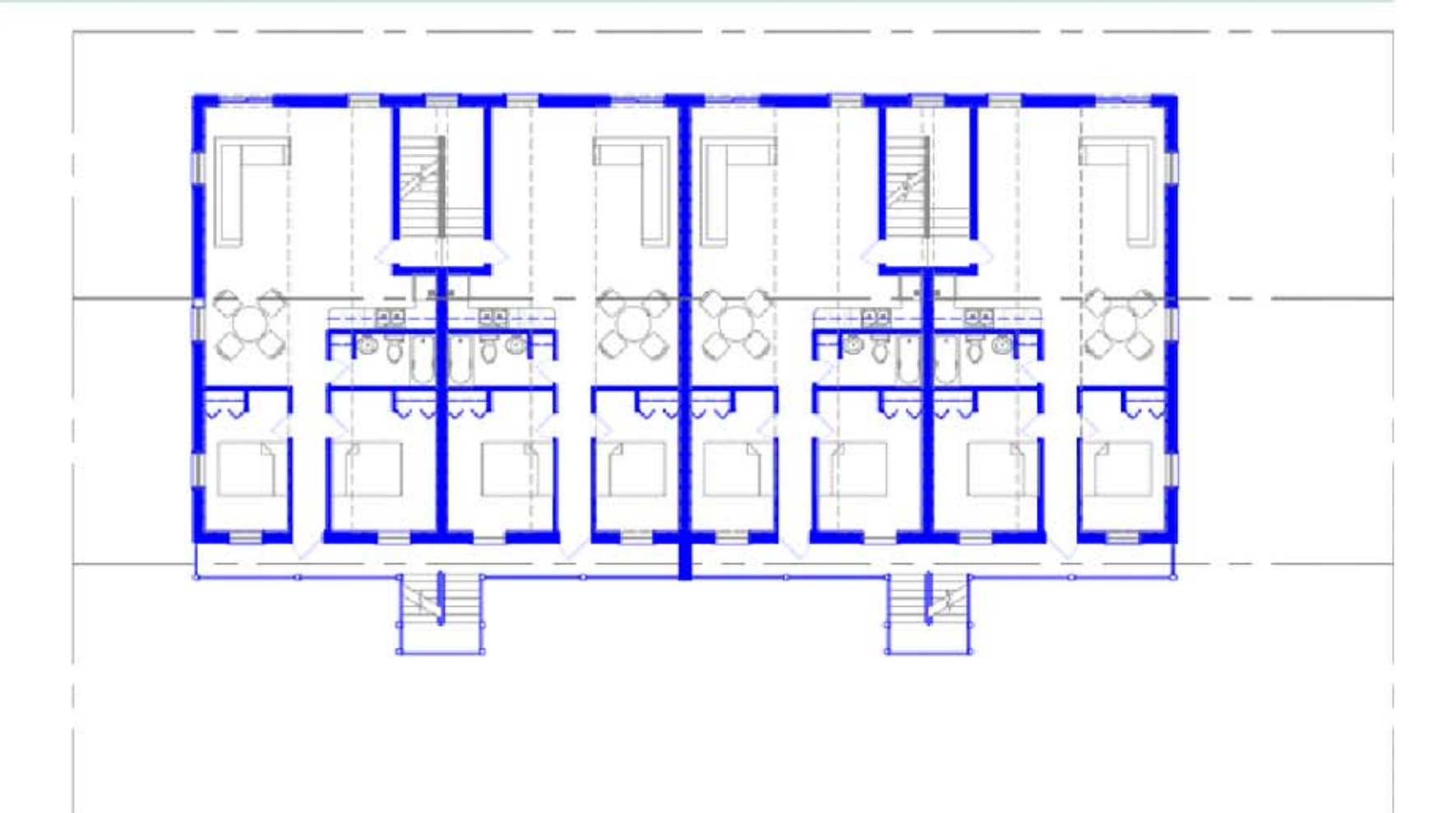
2nd & 3rd Level Floor Plan
