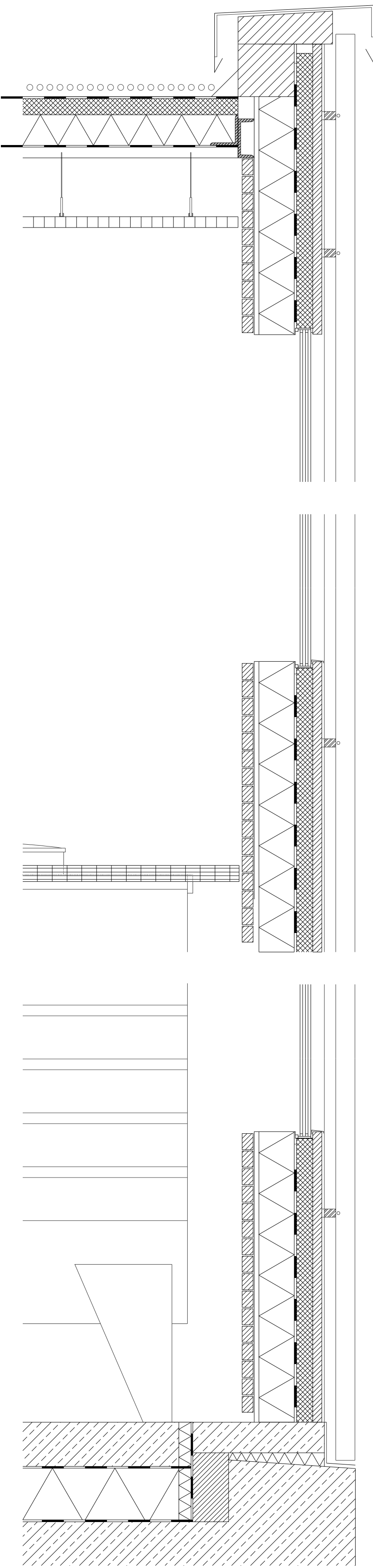
Wall Section
