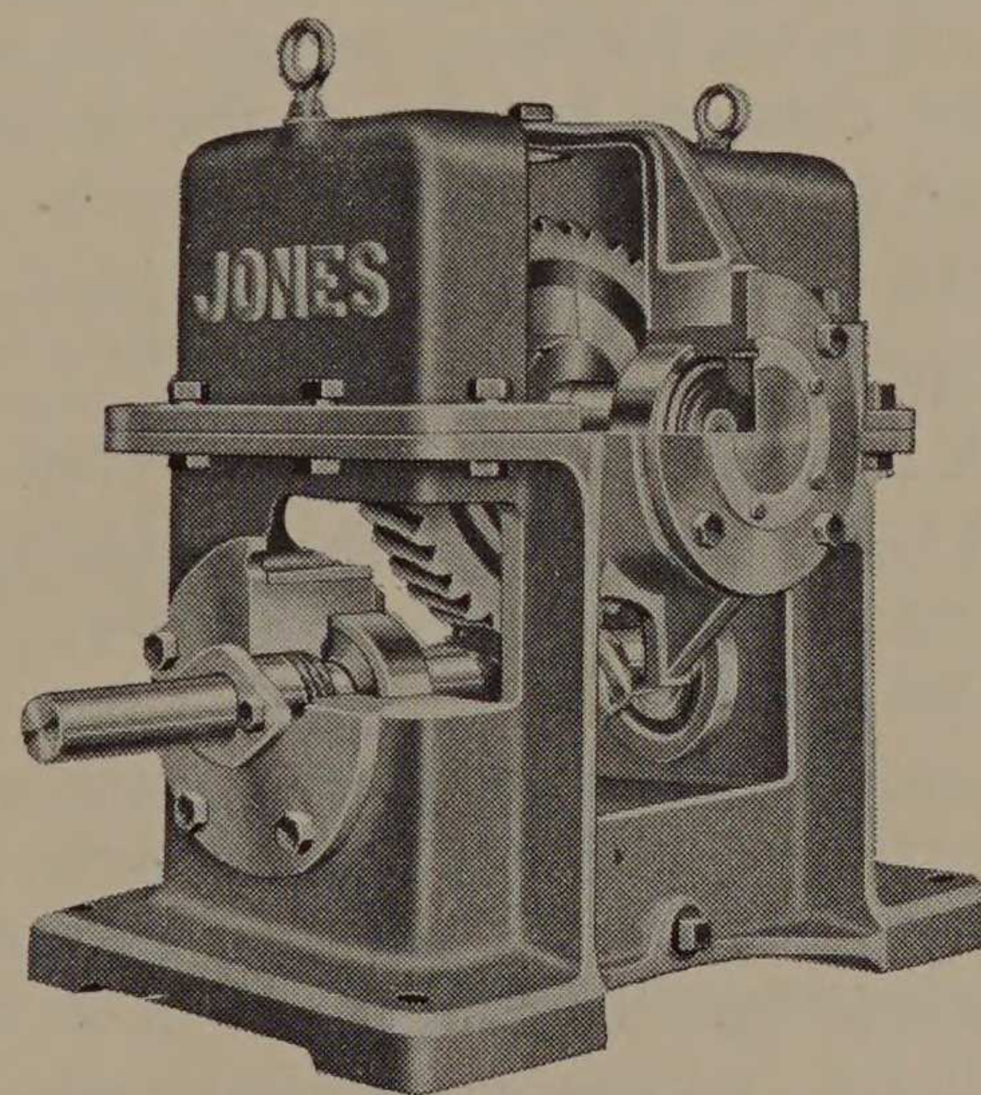
Jones Heavy-Duty Worm Gear Speed Reducer
