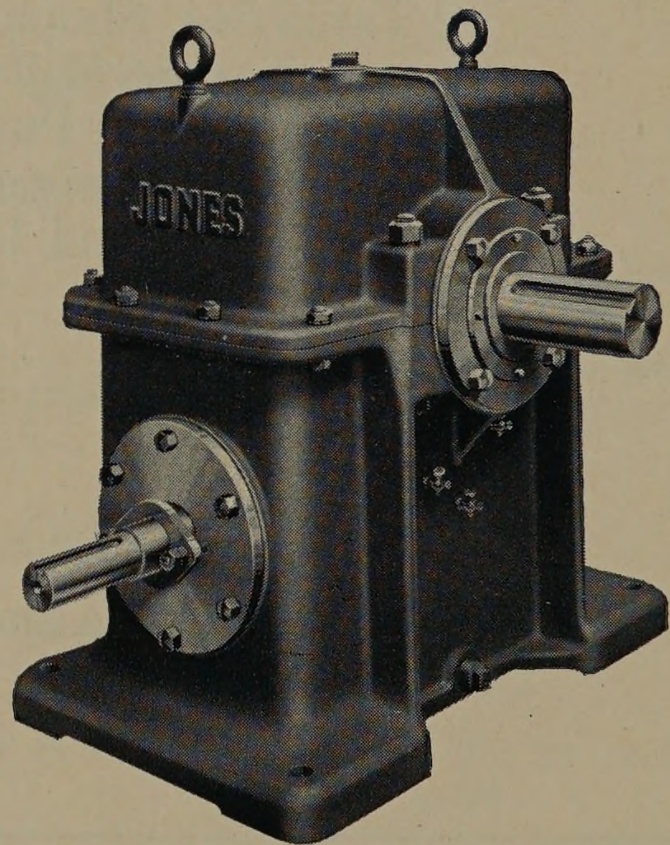
Jones Heavy-Duty Worm Gear Speed Reducer
