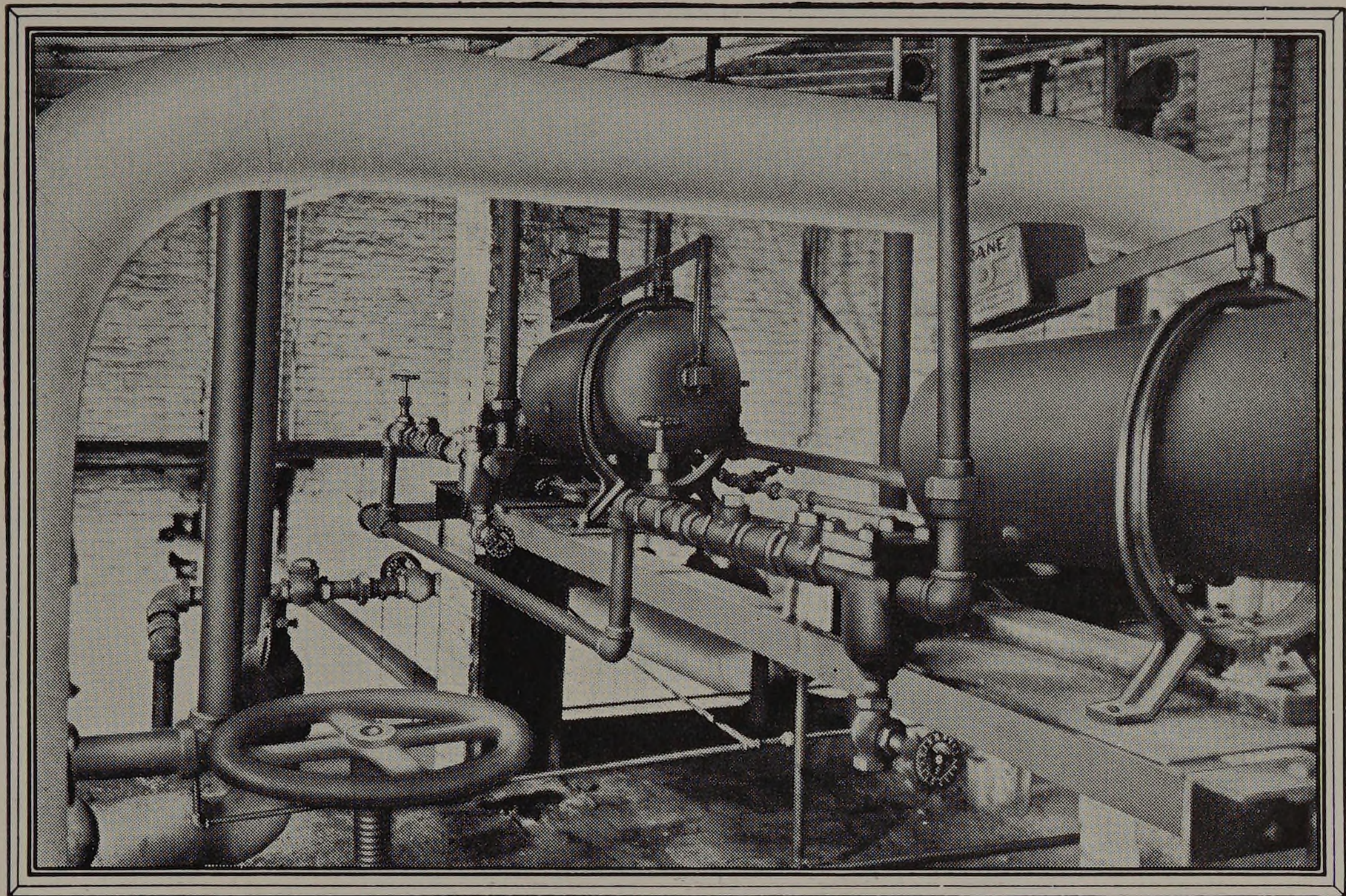
HOLLAND LAUNDRY, INC., PHILADELPHIA, SOLVED THEIR CONDENSATION AND BOILER FEED PROBLEMS WITH CRANETILT STEAM TRAPS. MR. WINTERSTEIN IS PLANT MANAGER
