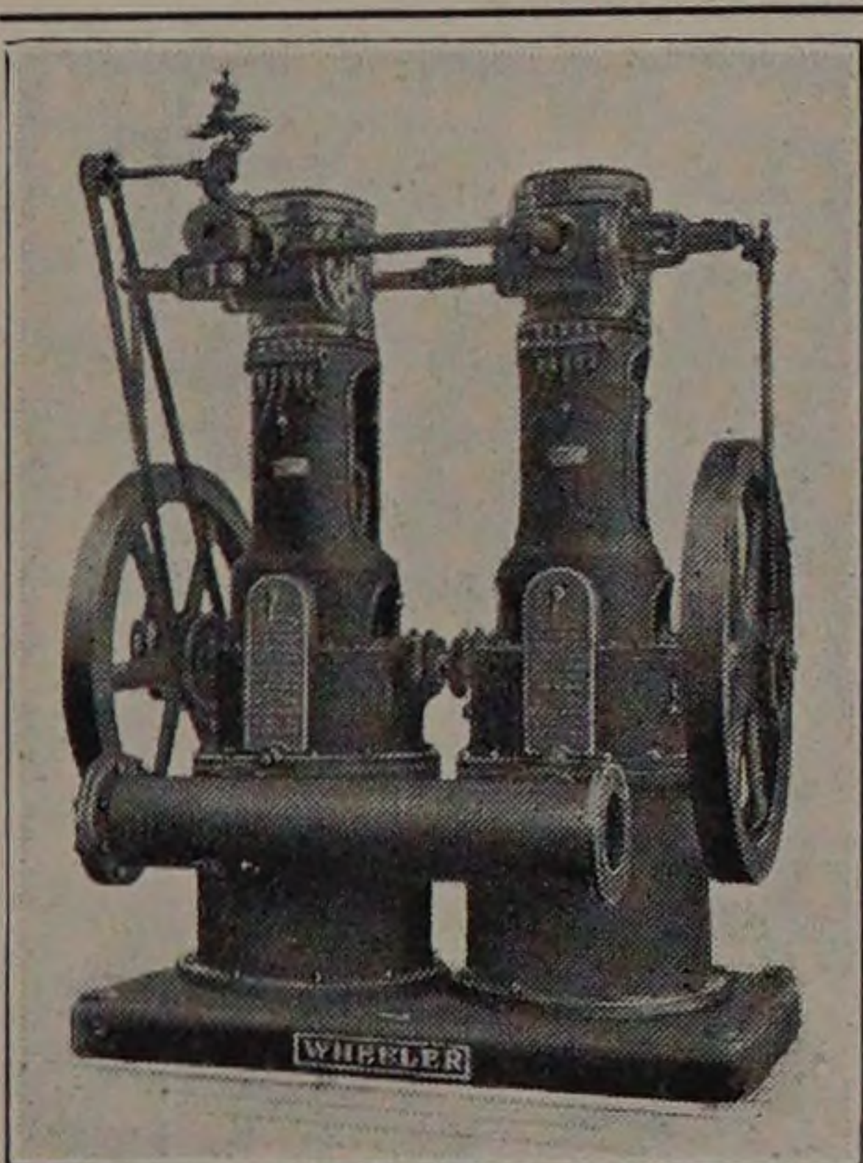
"Edwards" Patent Air Pump, Twin Type
