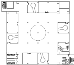
Parsi Section Floor Plans
